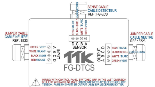
Figure 1.4.2.1: Addressable box FG-DTCS cabling diagram
