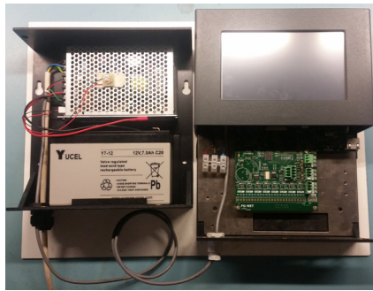
Example of connection between Battery backup and FG-NET digital unit
