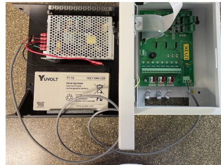
Example of connection between Battery backup and FG-SYS digital unit
