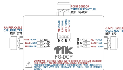
Figure 1.4.6 : Point sensor diversion box FG-DOP cabling diagram
