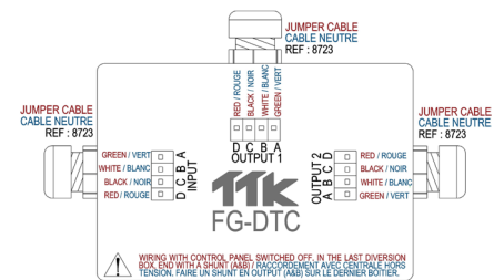
Figure 1.4.1.1: Diversion box FG-DTC cabling diagram
