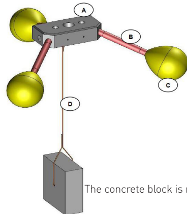
Wall-guided flotation system
